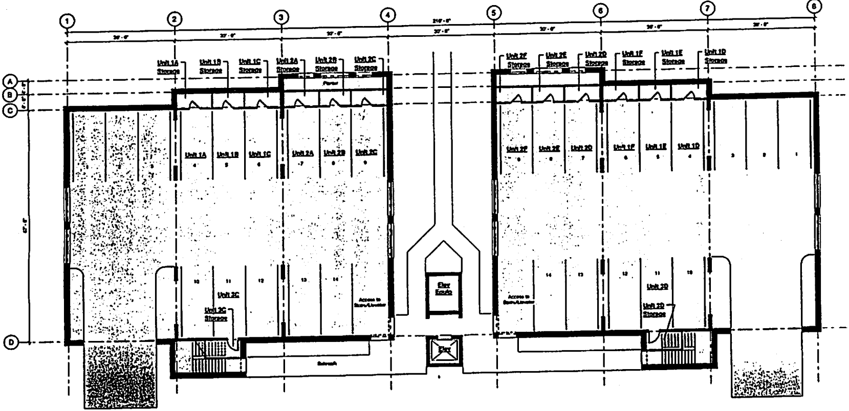
Overall Ground Level Garage Plan
